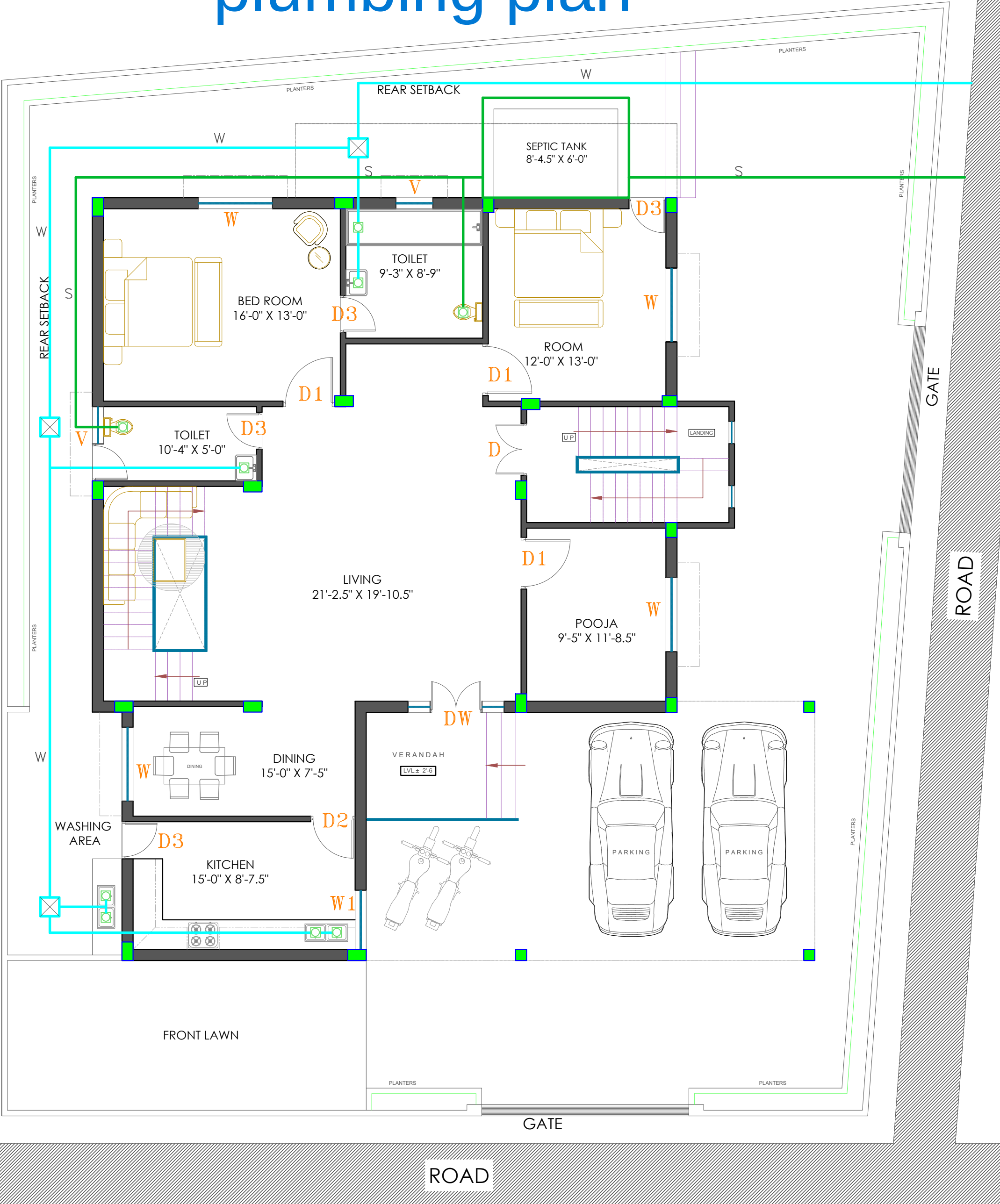
GROUND FLOOR PLUMBING PLAN
