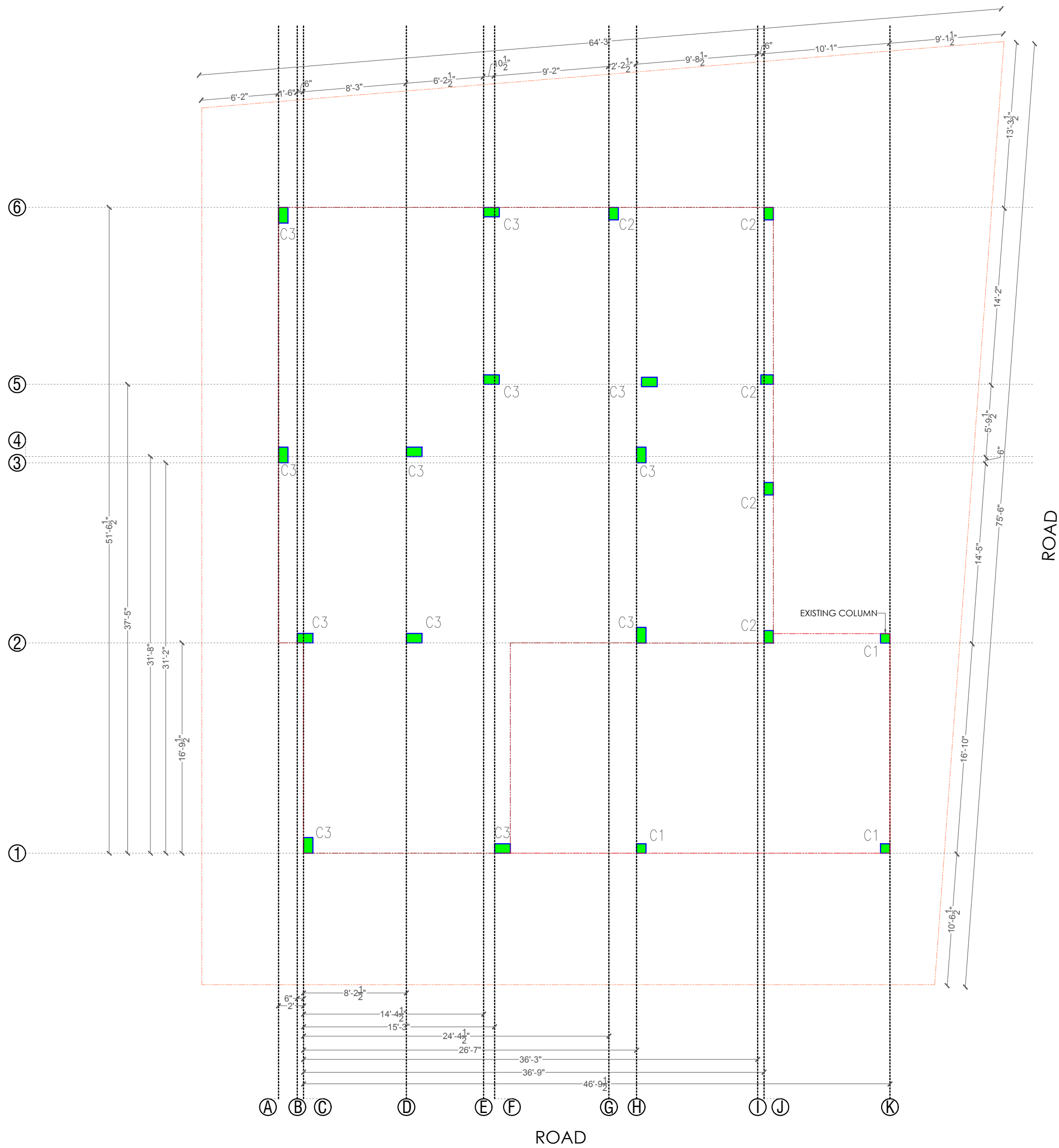
COLUMN CENTERLINE PLAN
